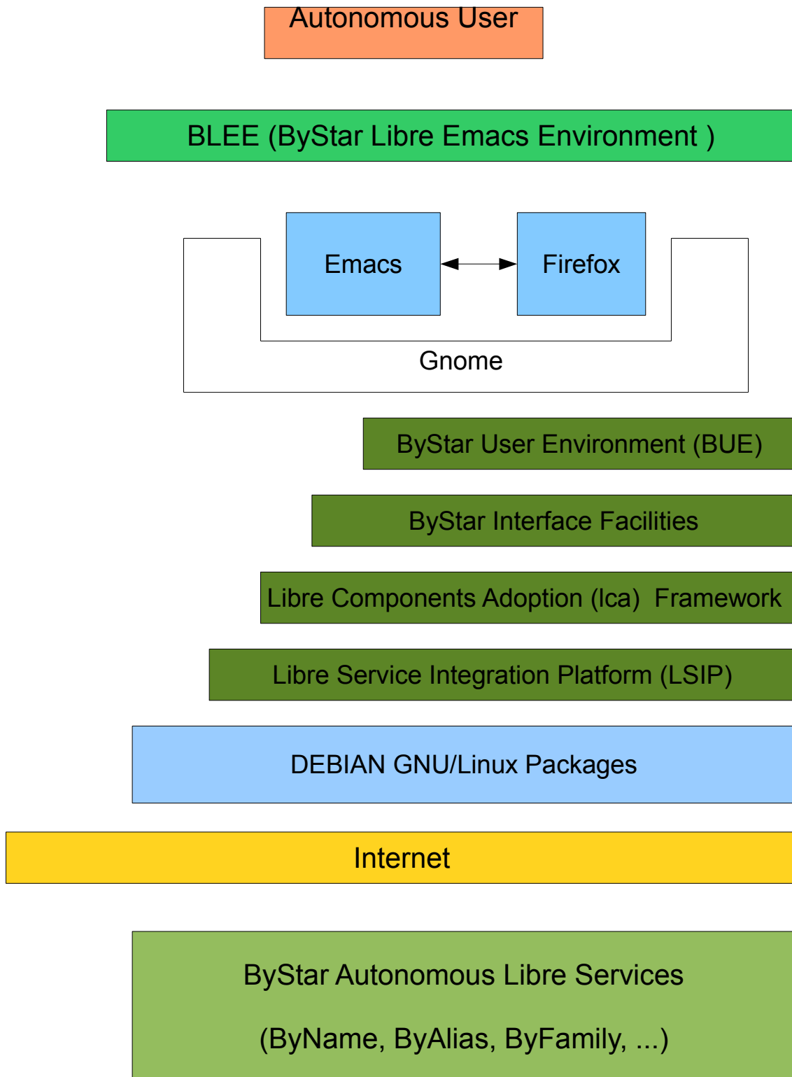
Figure 3: BleeModel
