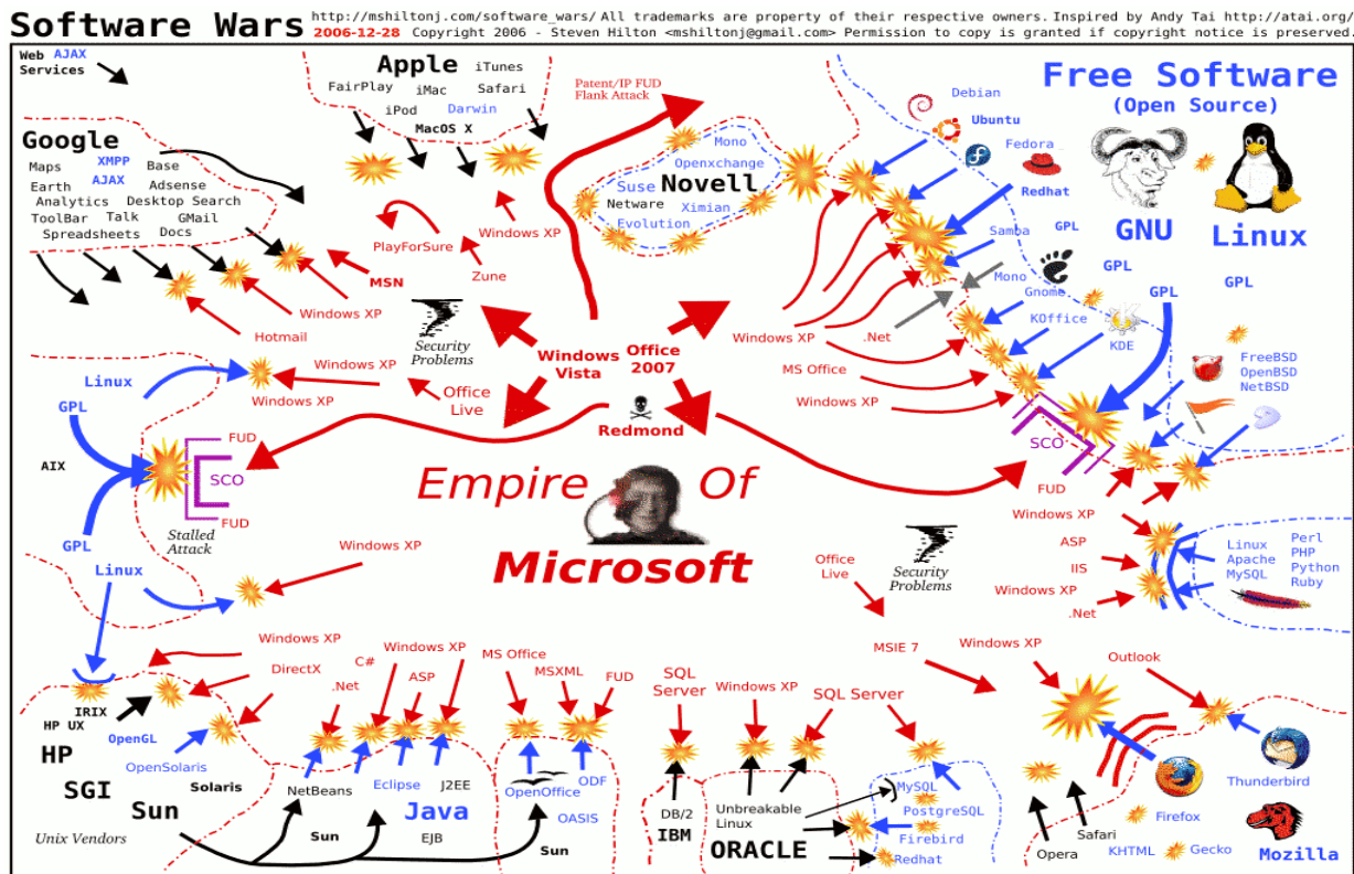
Figure 20: softwareWars
