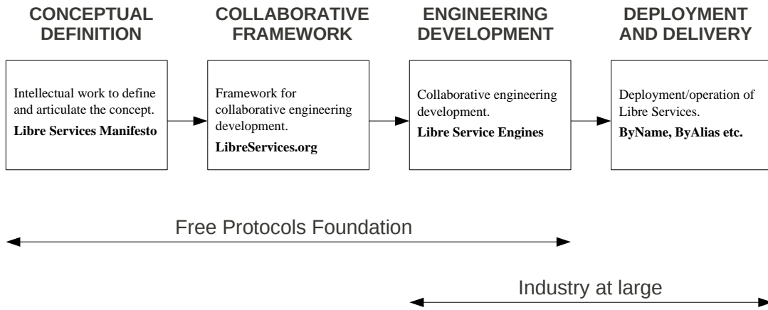
Figure 9: conceptToDeliveryCollab
