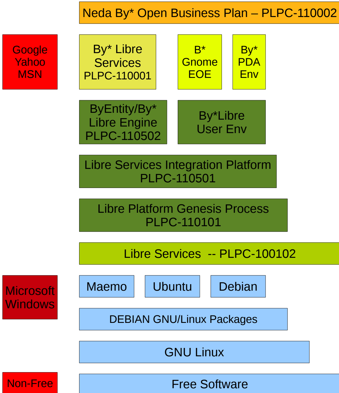
Figure 16: LS-LayersMinusTexting
