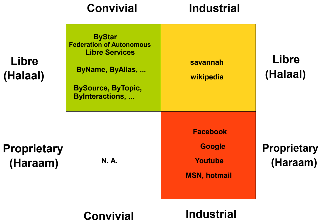
Figure 10: convivialServicesQuadrant
