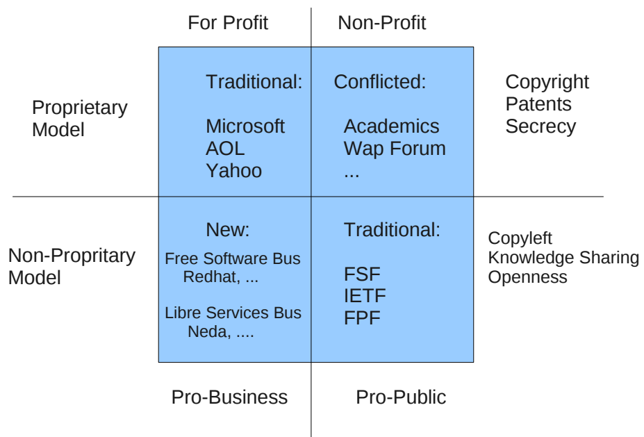
Figure 12: forProfitNonProprietaryQuadrant
