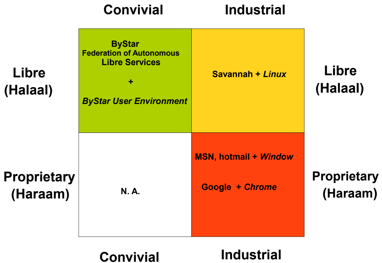
Figure 11: convivialSoftwareServicesQuadrant
