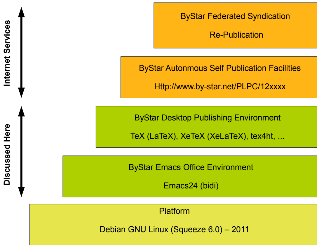
Figure 18: publicationLayers
