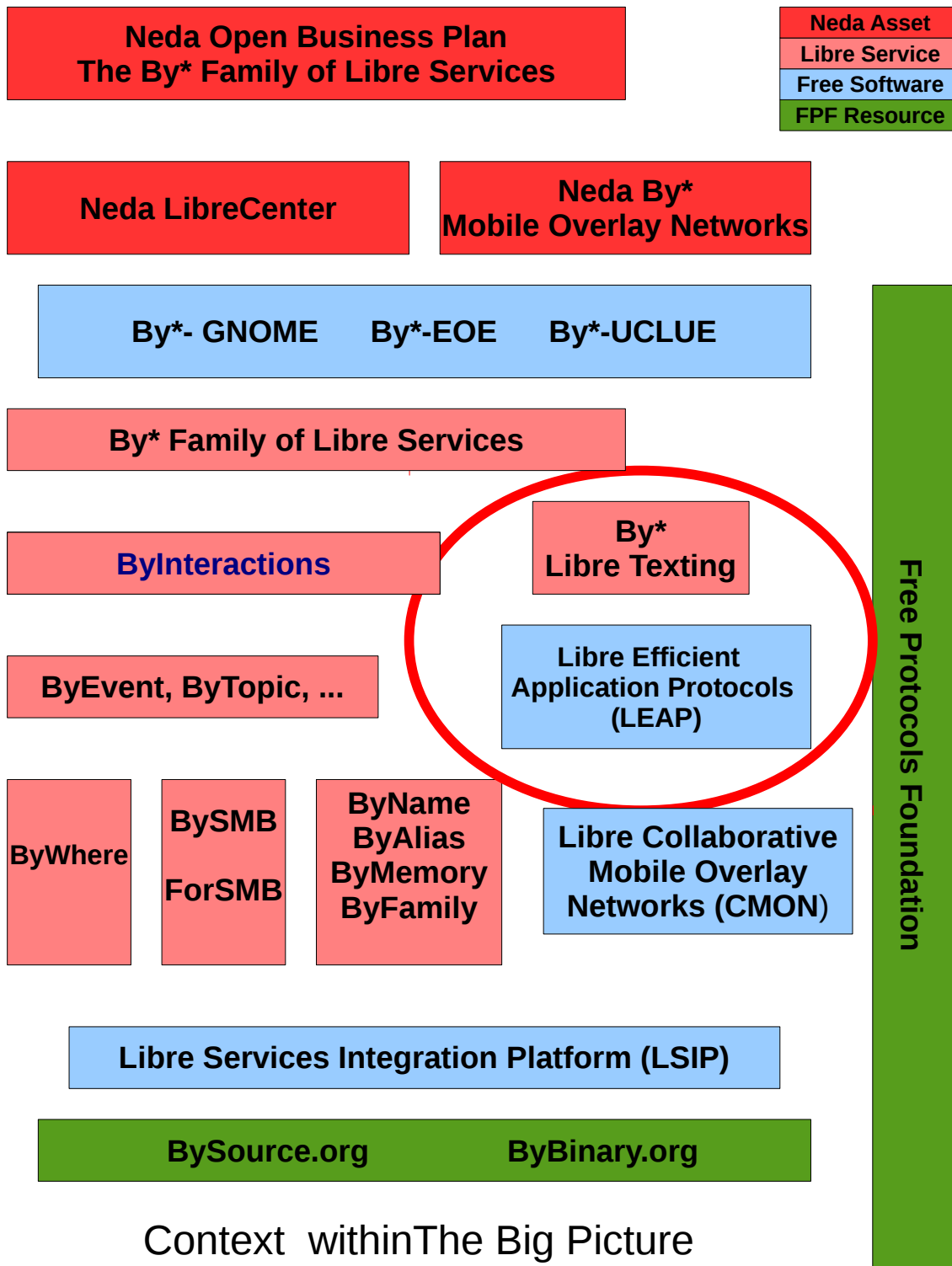
Figure 17: LT-Context
