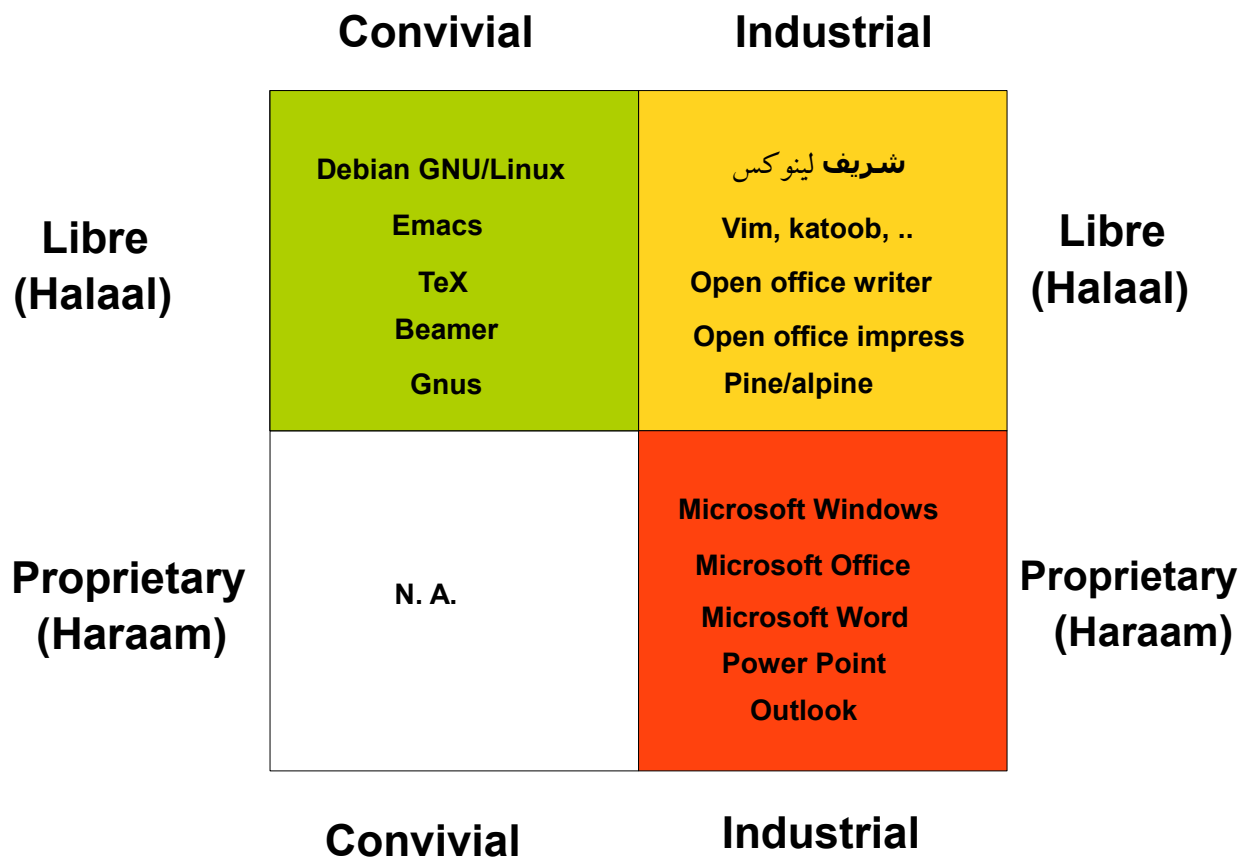
Figure 14: libreConvivialQuadrant
